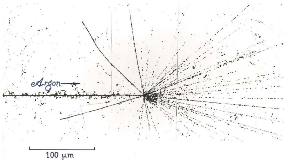
Figure 4. High energy Argon ion moving through photographic material. Photograph courtesy of Lawrence Berkeley National Laboratory.
