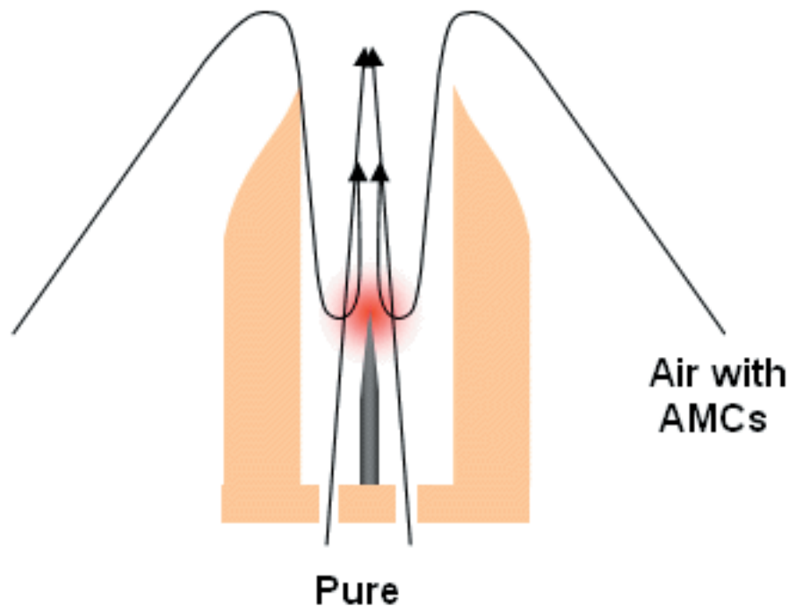
Figure 3. Design trap of a sheath nozzle design.
